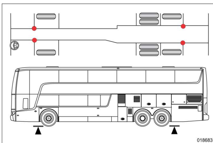
Detail of jacking point
